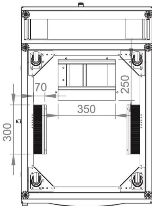
Bottom view
