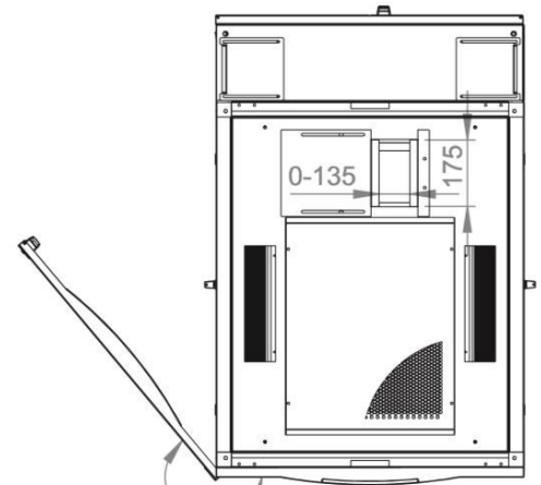
0°-230° Front door opening angle
