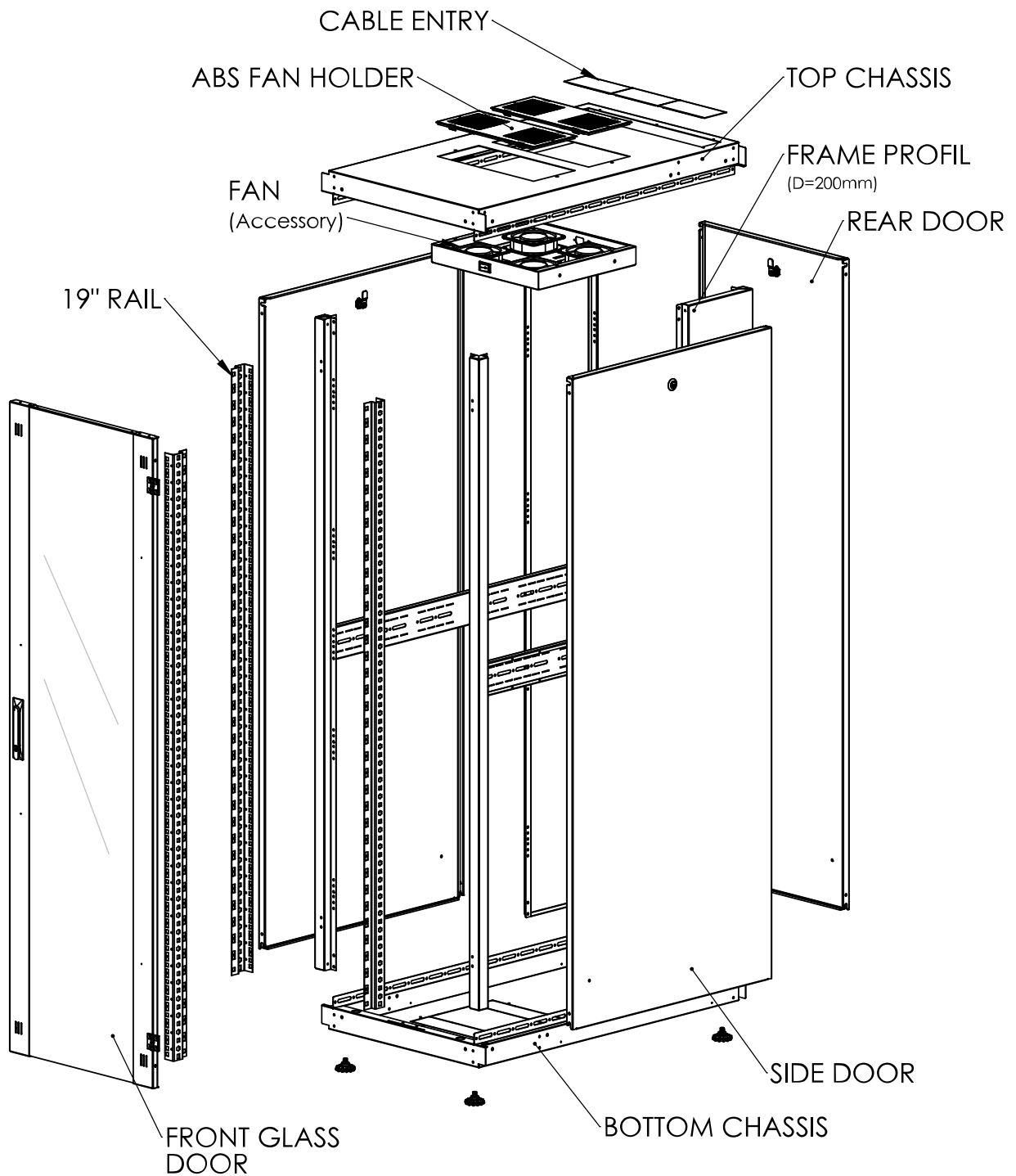
Exploded view
